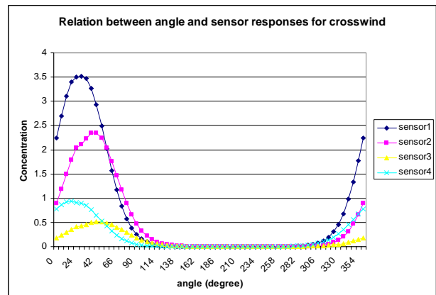
Fig. 4 Relations between angle \theta and sensors responses for crosswind case
