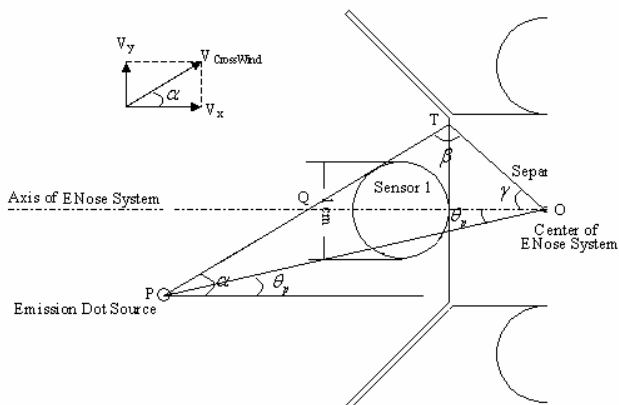
Fig. 6 Calculation of angle for peak point
