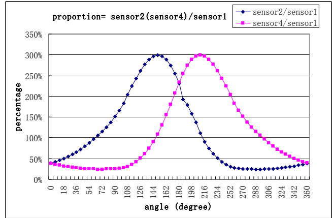
Fig. 3 Ratio of C2/C1 and C4/C1
