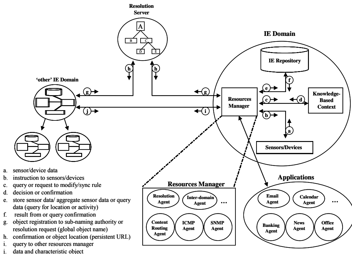
Figure 3.3 DiCPA: Distributed Context Processing Architecture for an Intelligent Environment
