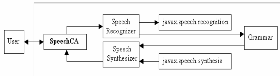
Figure 4.6 Block Diagram Speech Context-aware Prototype
