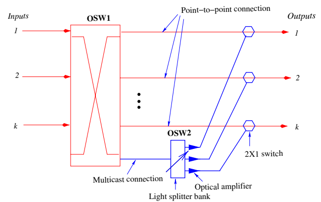
Fig. 1 Light splitter-sharing switch [2]
