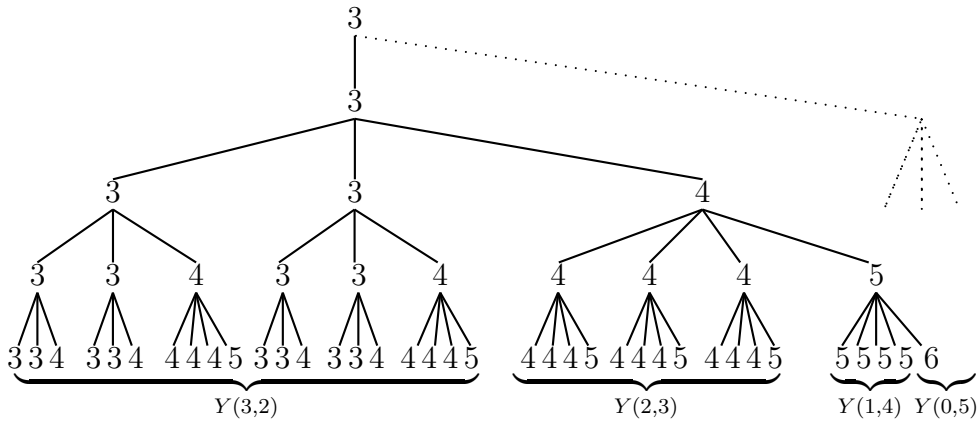
Figure 1: One branch of Y(4, 2) initially rooted at 3.
