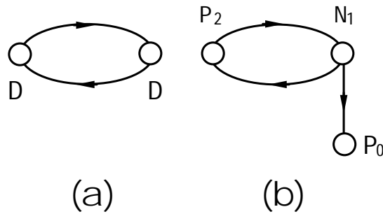
FIGURE 2. Games on simple cyclic digraphs.
