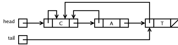
Figure 2: Linked-list representation. Each disjoint set can be represented by a linked-list. Each node has a pointer to the head node and a pointer to the next node.
