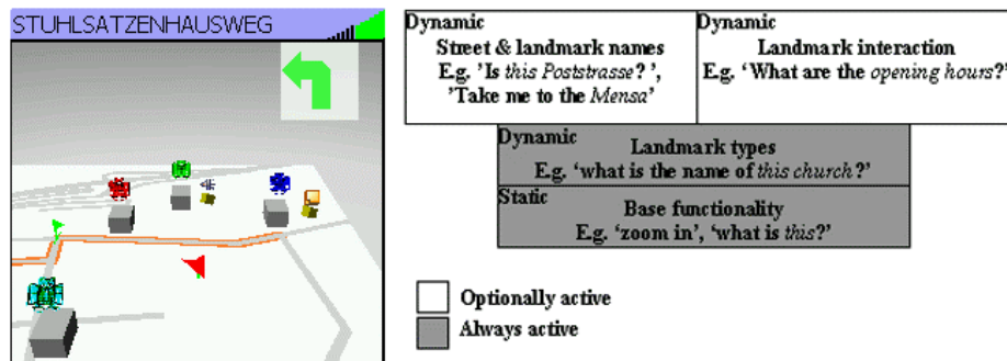
Fig.1. Static and dynamic speech grammars, and a PDA screen-shot of a route containing landmark interaction objects
