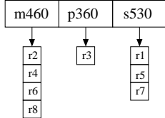
Figure 2: Standard blocking index resulting from the example records given in Figure 1. The blocking keys correspond to Soundex encodings.
