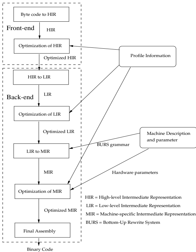
Figure 3: Internal structure of Jalapeño Optimizing Compiler for compiling a single method
