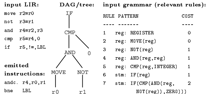
Figure 10: Example of tree pattern matching for PowerPC
