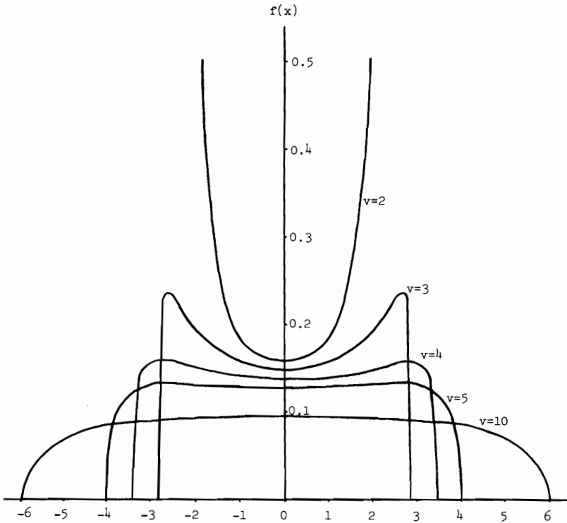
FIG. 1. Limiting eigenvalue densities for various v .
