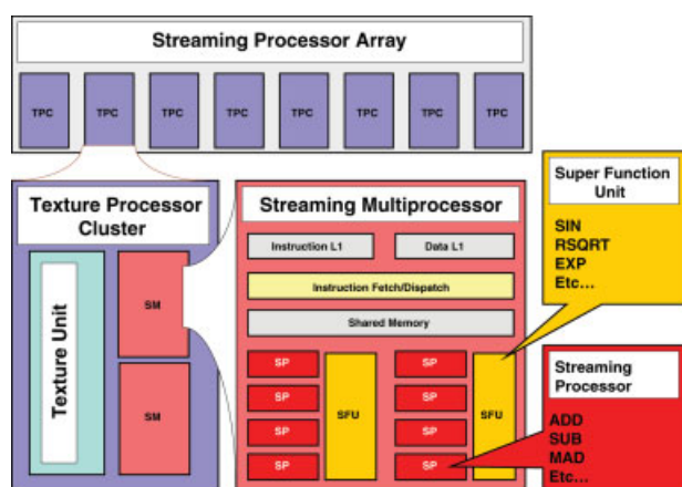
Figure 1. NVIDIA G80 hardware block diagram. 241 \times 172 mm ( 600 \times 600 DPI). [Color figure can be viewed in the online issue, which is available at www.interscience.wiley.com .]
